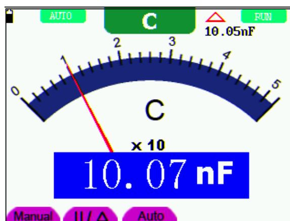
figure 24: Capacitance Measurement
