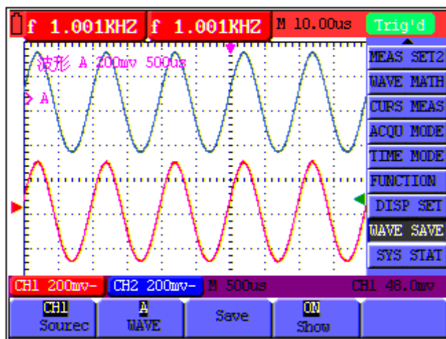
figure 43: Waveform Saving
