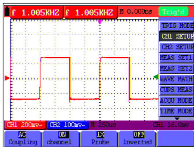
figure 35: AC Coupling
