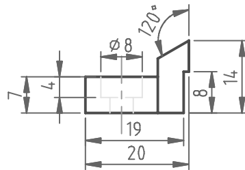
Gradenaanduiden Degrees pointer
